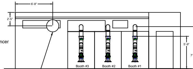
26" Louver East Elevation Interior
