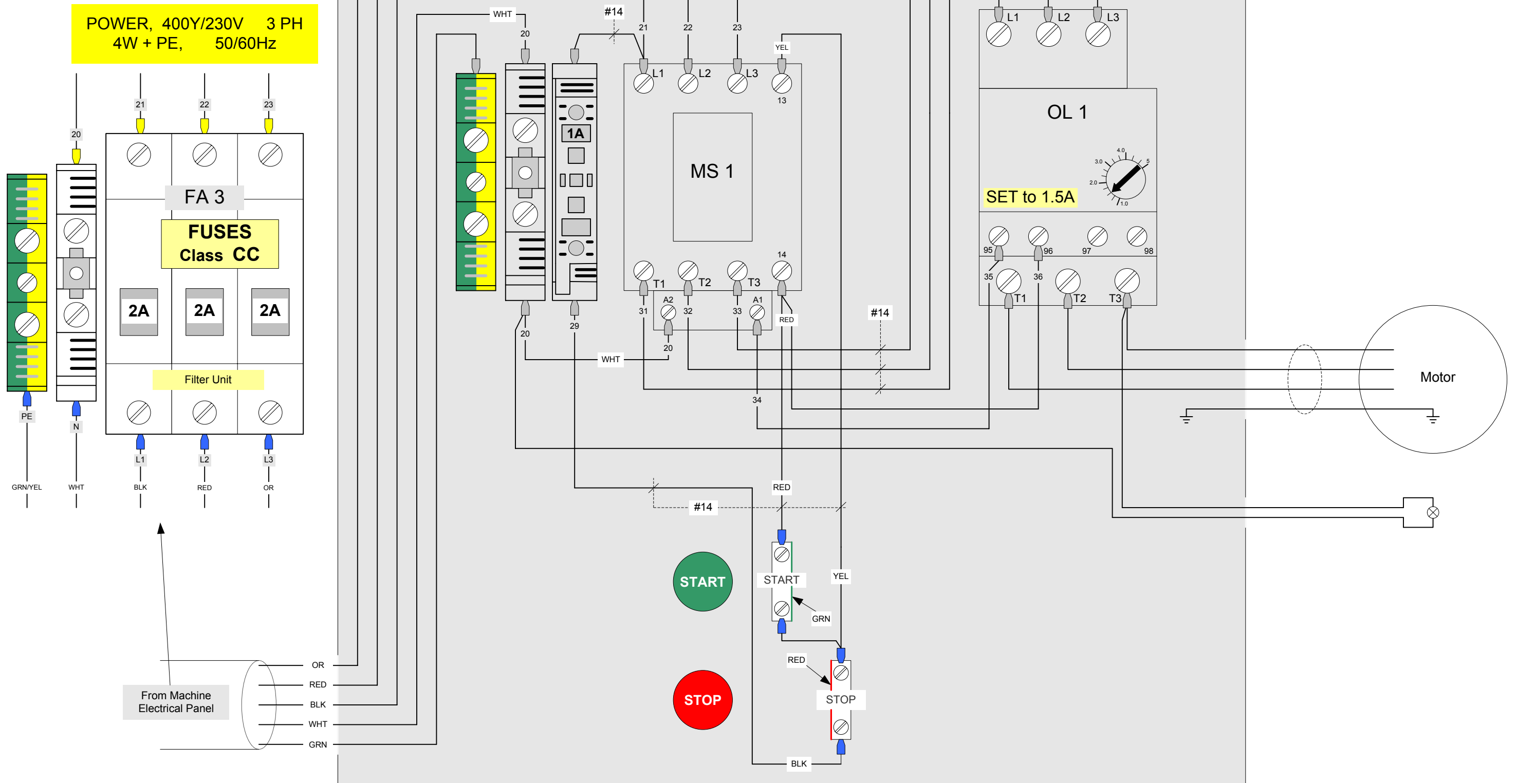
Jeti 3324WBT Filter Unit Wiring
