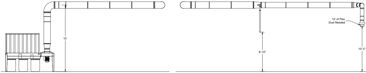
Elevation View
