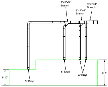
Elevation View Section A-A
