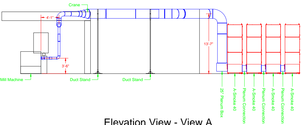
Elevation View - View A
