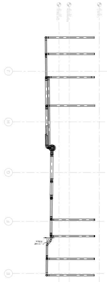
③ Exhaust Dust Grinding Section 2 1/8" = 1'-0"
