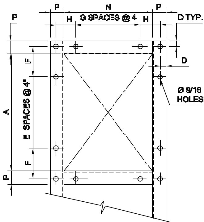
FLANGED OUTLET
