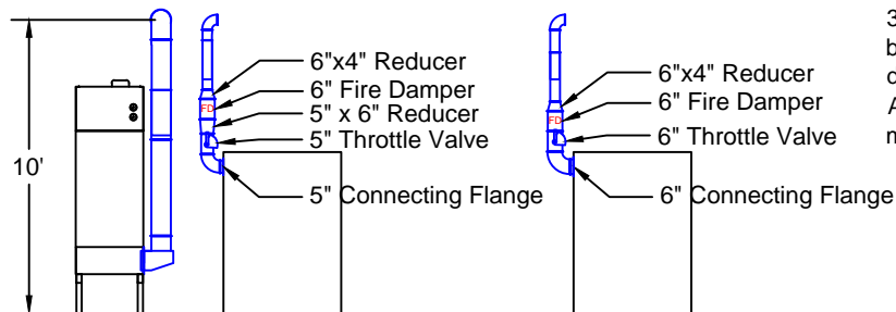
Elevation View
