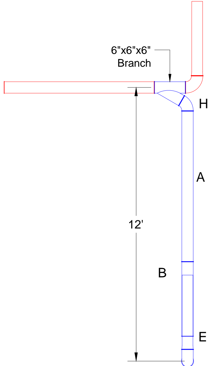
Plan View - Future Install
