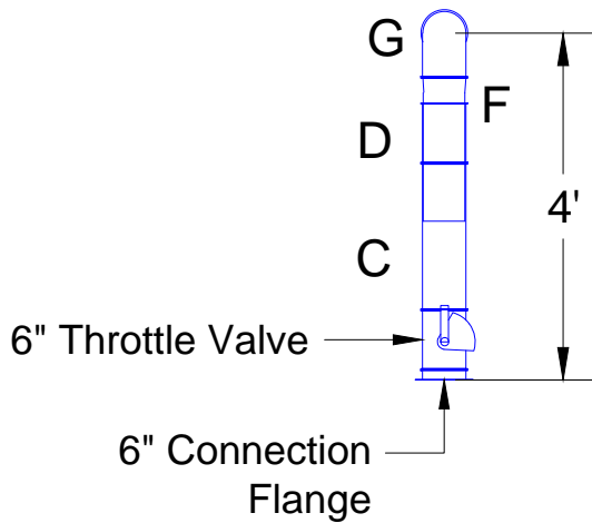
Elevation View - Future Install
