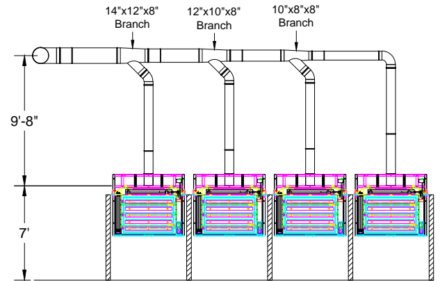
Elevation View
