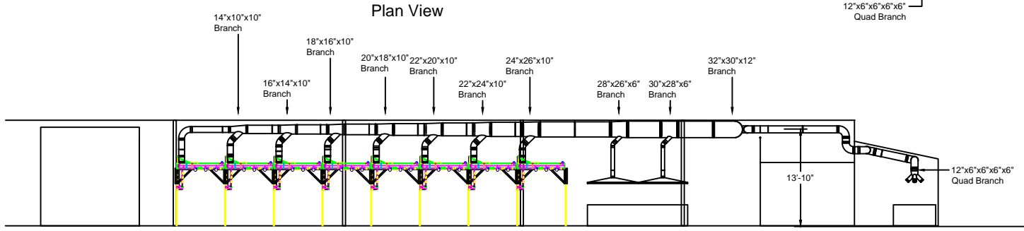
Elevation View - SDC-AT-4-48
