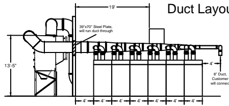
Elevation View - South Side
