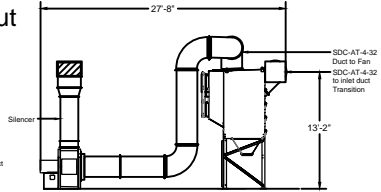
Elevation View - North Side
