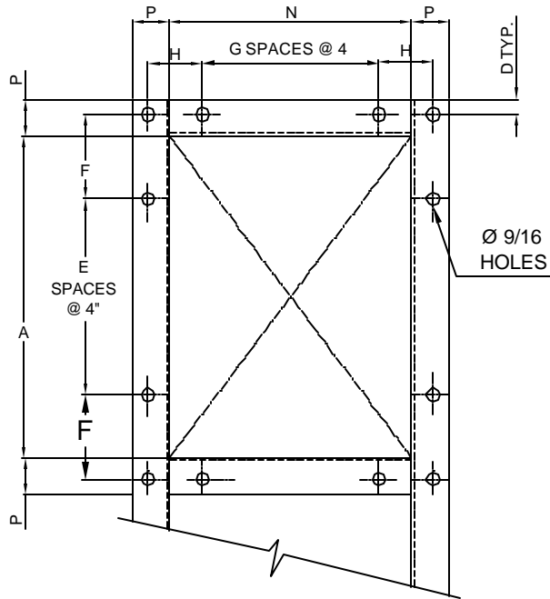
FLANGED OUTLET
