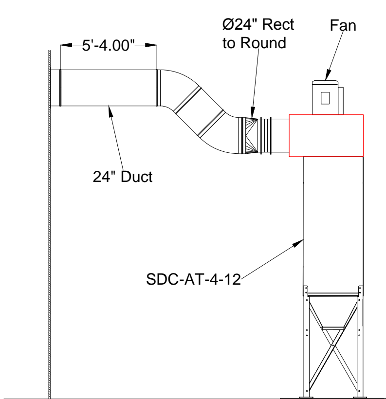
Current Layout
