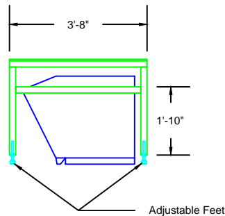
Adjustable Feet
