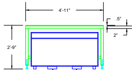
Forklift Pockets 22"L x 7"W x 2"H
