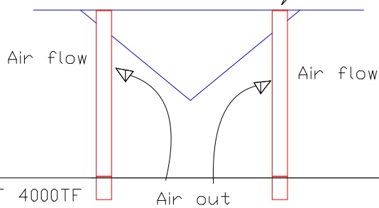
Side View of Air Diverter Plate
