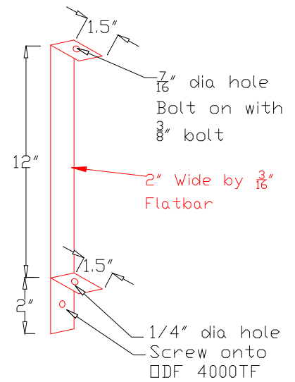
View of Legs Typical of 4
