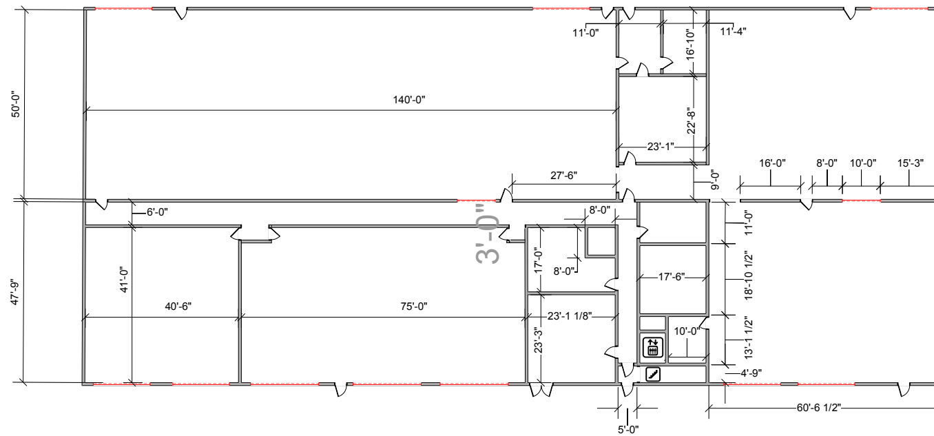
TOP (MIDDLE SECTION) VIEW
