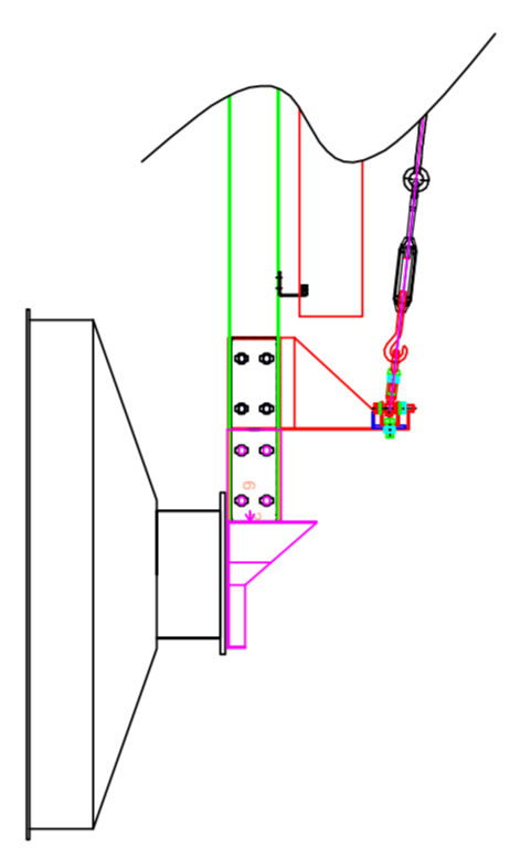
TYPICAL 48" BY 48" HOOD CONNECTION DETAIL A (SCALE 2 TO 1)
