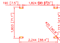
PLAN DETAIL
