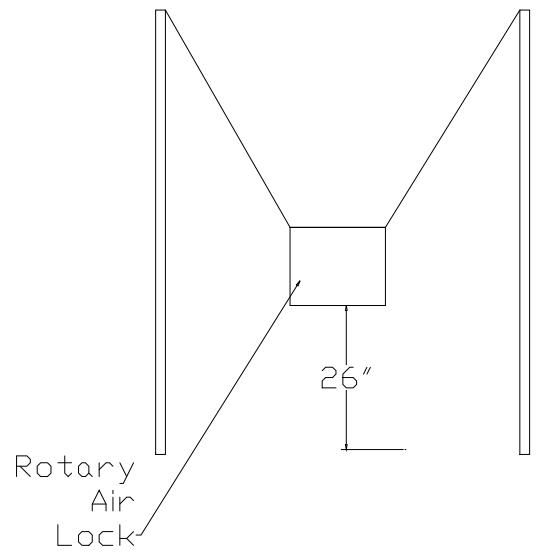
Side View of Bottom Hopper section
