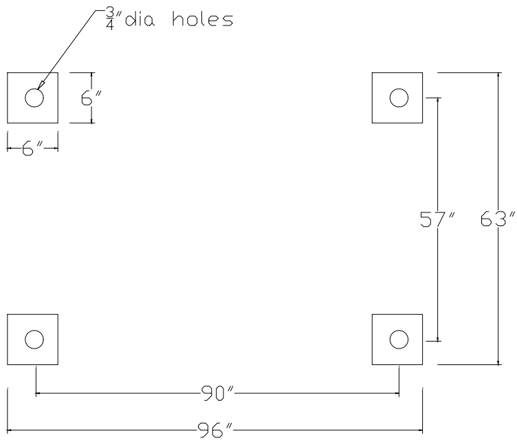
Plan View of Dust Collector footprint
