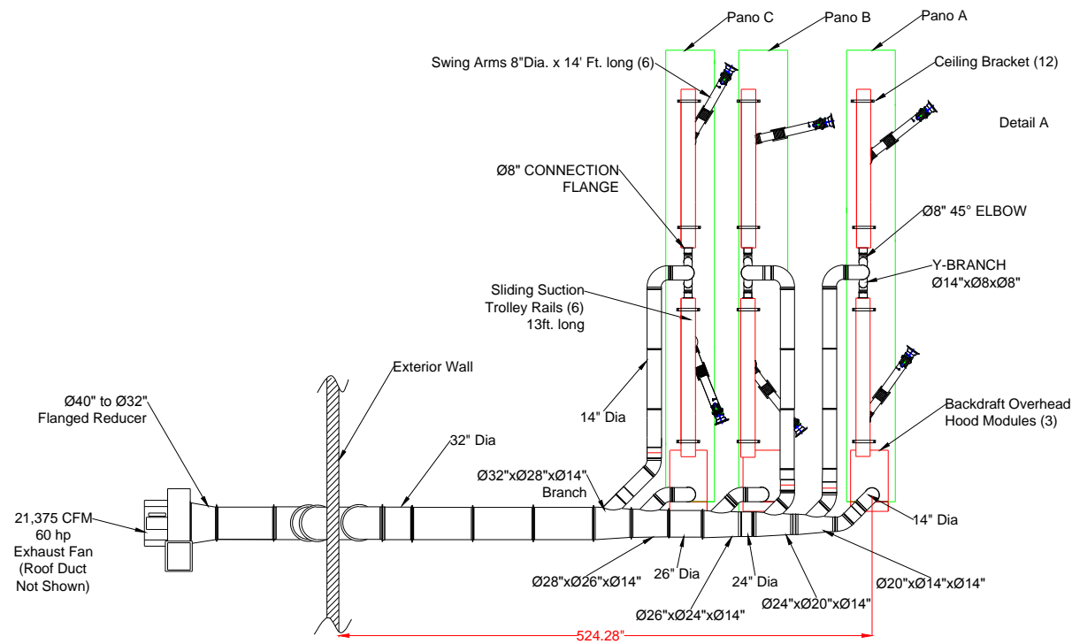
Plan View
