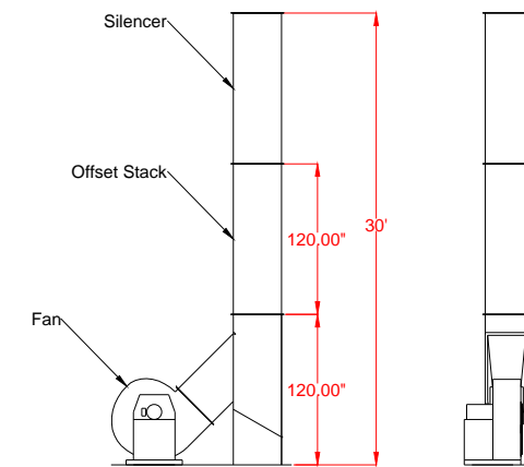
Elevation View Offset Stack
