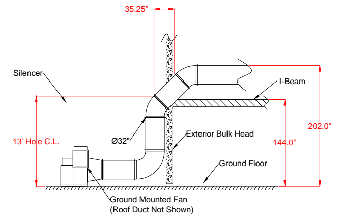
Elevation View Main Trunk Line
