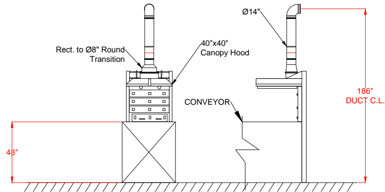
Front Side Elevation Back-draft Canopy Hoods (scale 2 to 1 for clarity)
