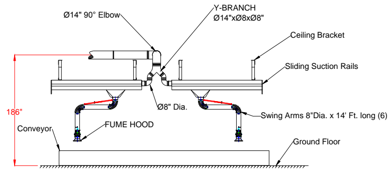
Elevation View Trolley Rail
