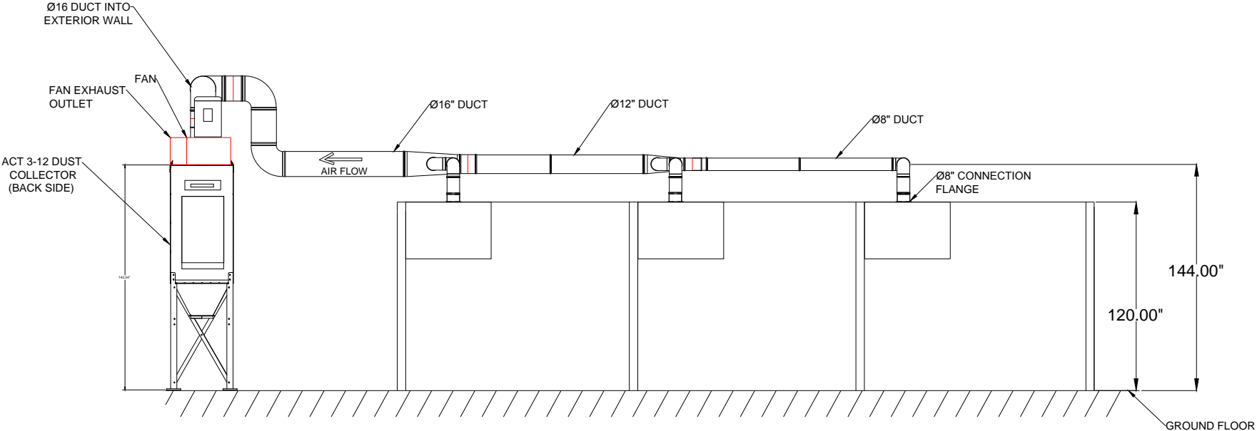
ELEVATION VIEW
