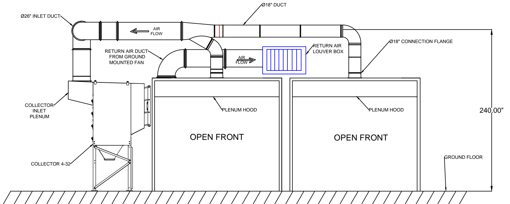
I.D. GRINDING-CLEANING STATION FRONT ELEVATION VIEW (EXTERIOR WALL NOT SHOWN)
