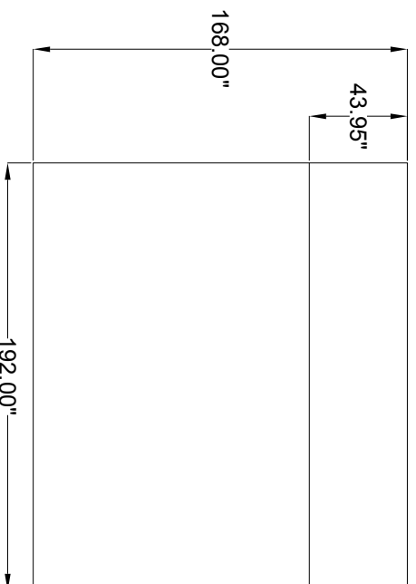
PLAN VIEW
