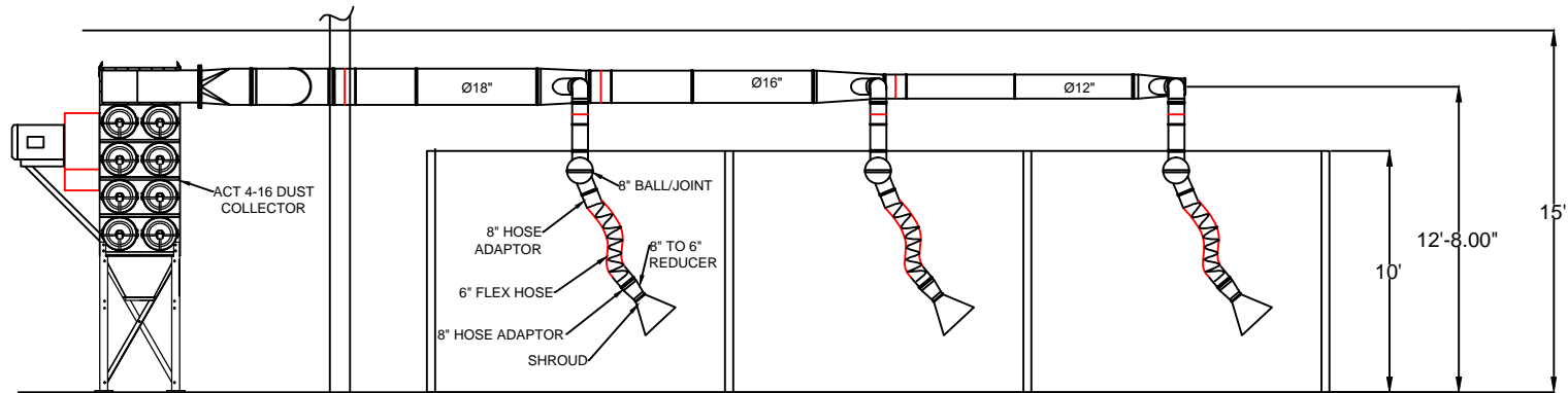
ELEVATION VIEW
