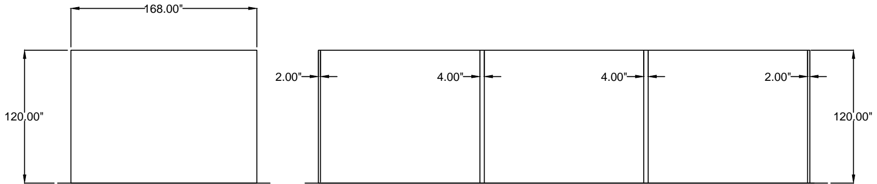
ELEVATION VIEW
