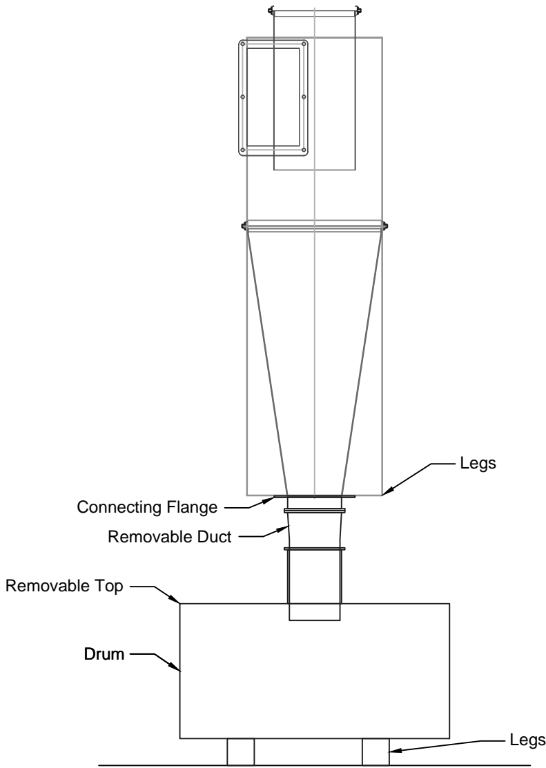
Assembly View
