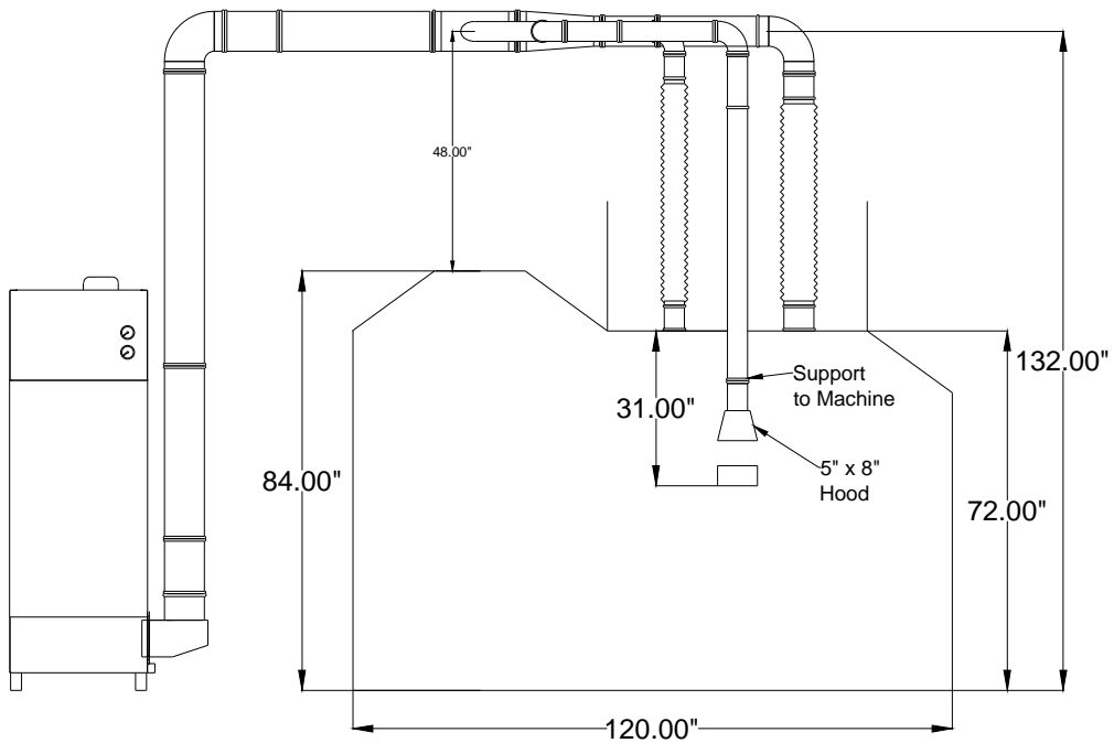
Elevation View
