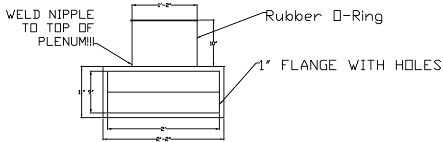
End View
