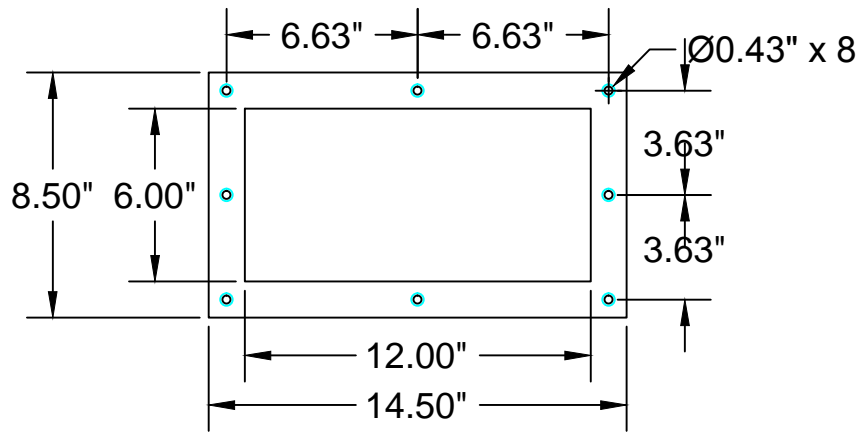
Flange View
