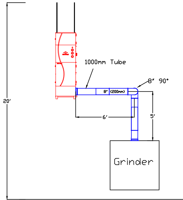
Elevation View
