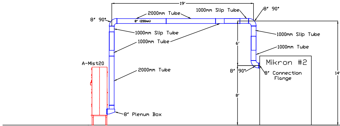
Elevation View
