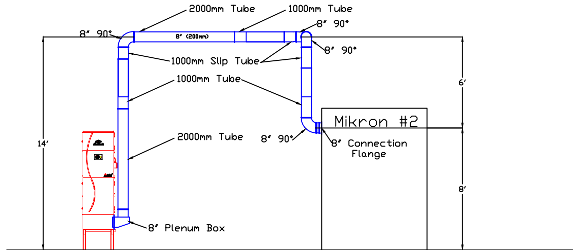
Elevation View
