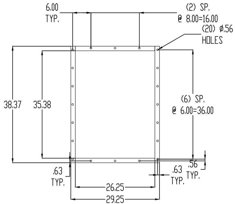
RECT FLANGE DETAIL
