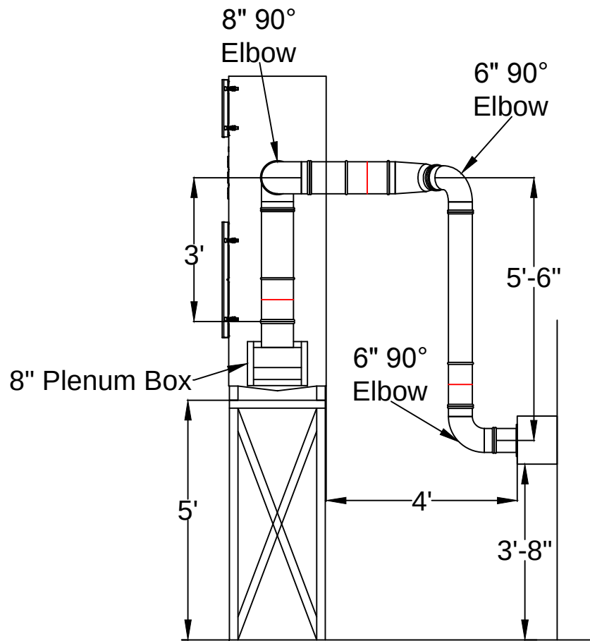
Elevation View
