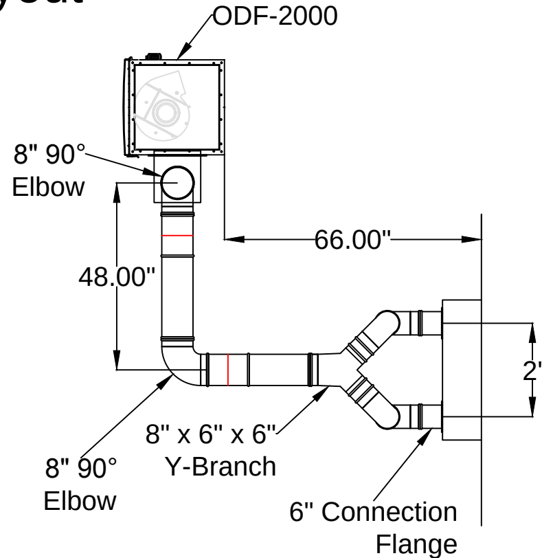
Top View
