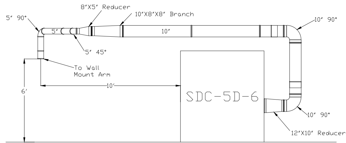
Elevation View Customer Enclosure Side
