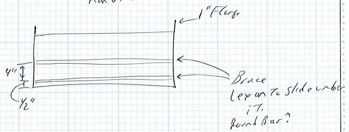
Plan View
