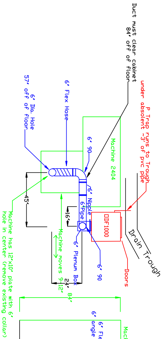
Plan View
