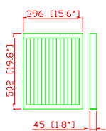
Pre-Primary Filter
