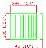
Synthetic Fiber Filter
