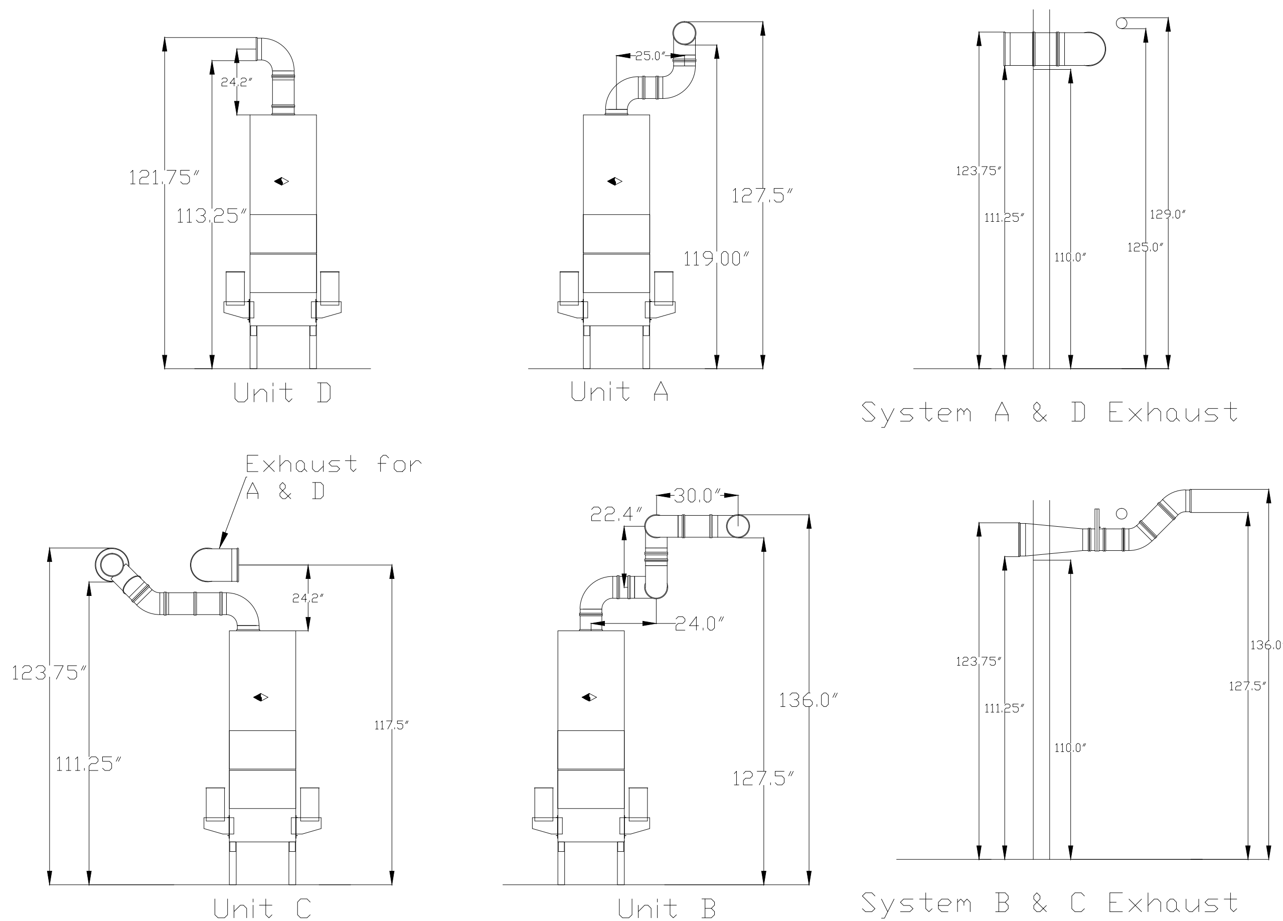
Elevation View
