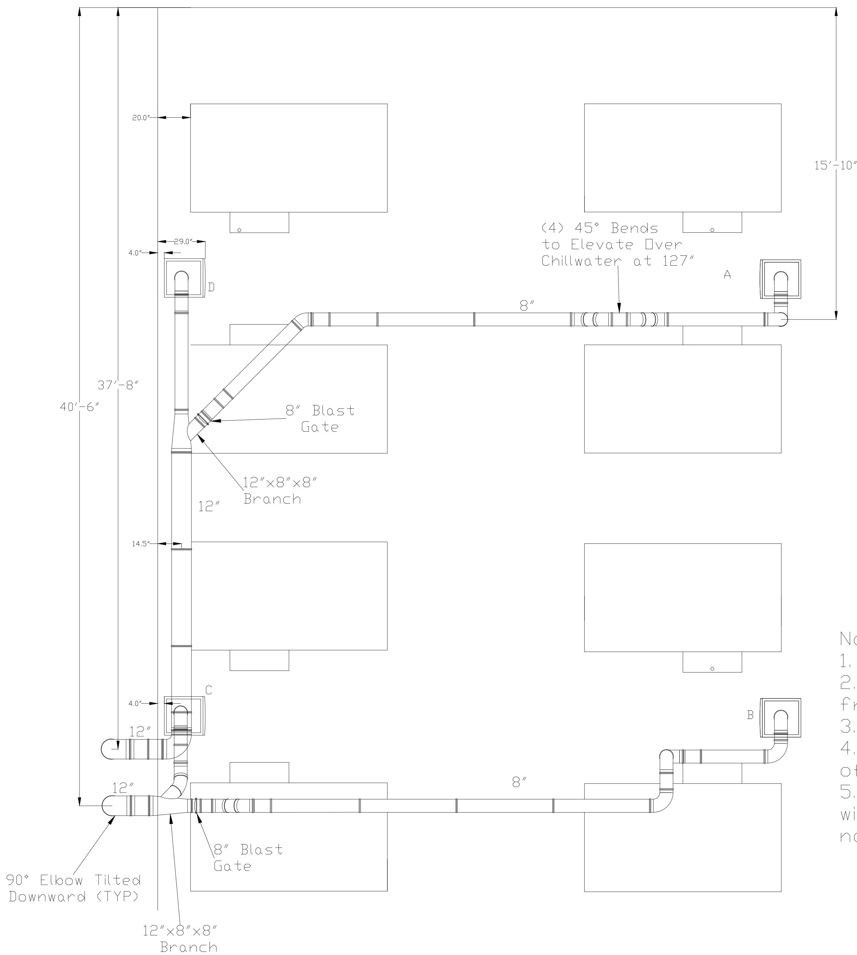
Plan View
