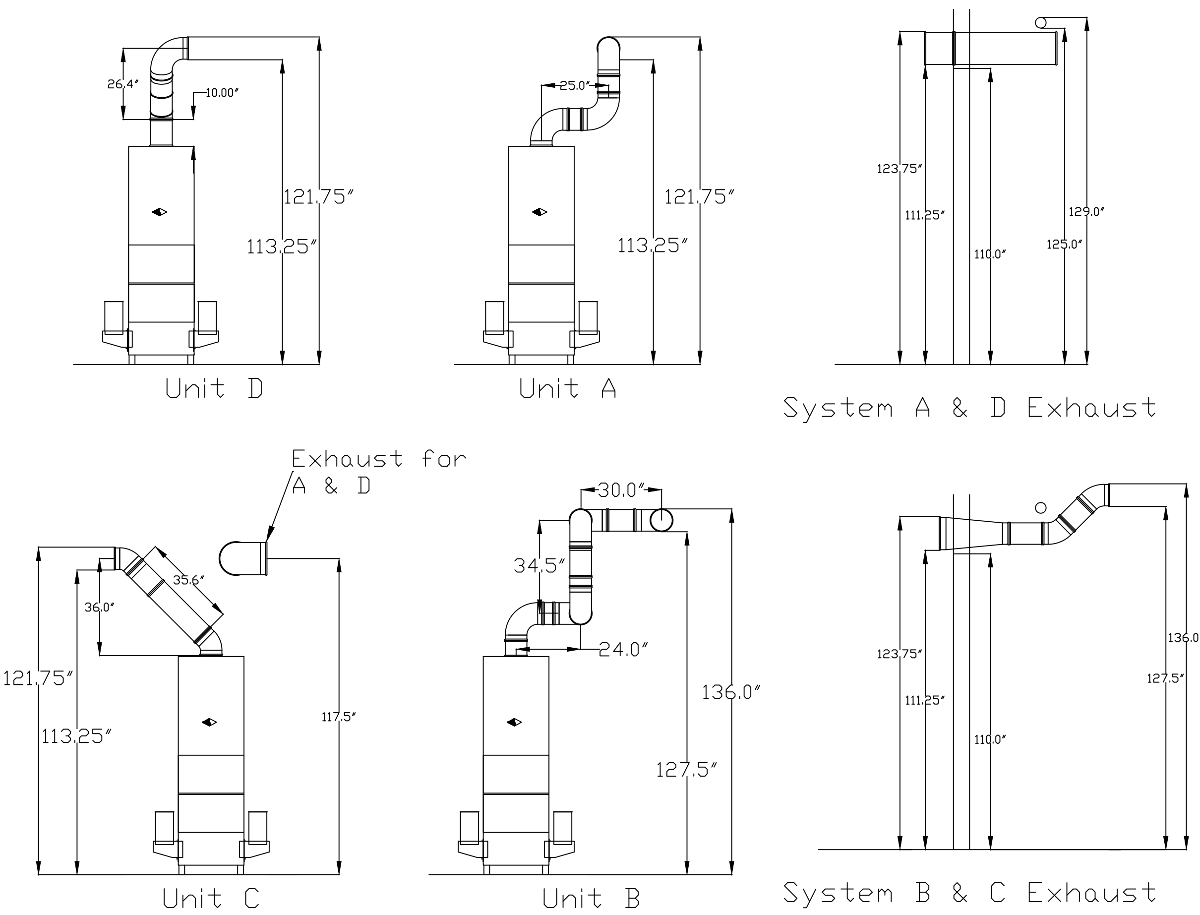
Elevation View
