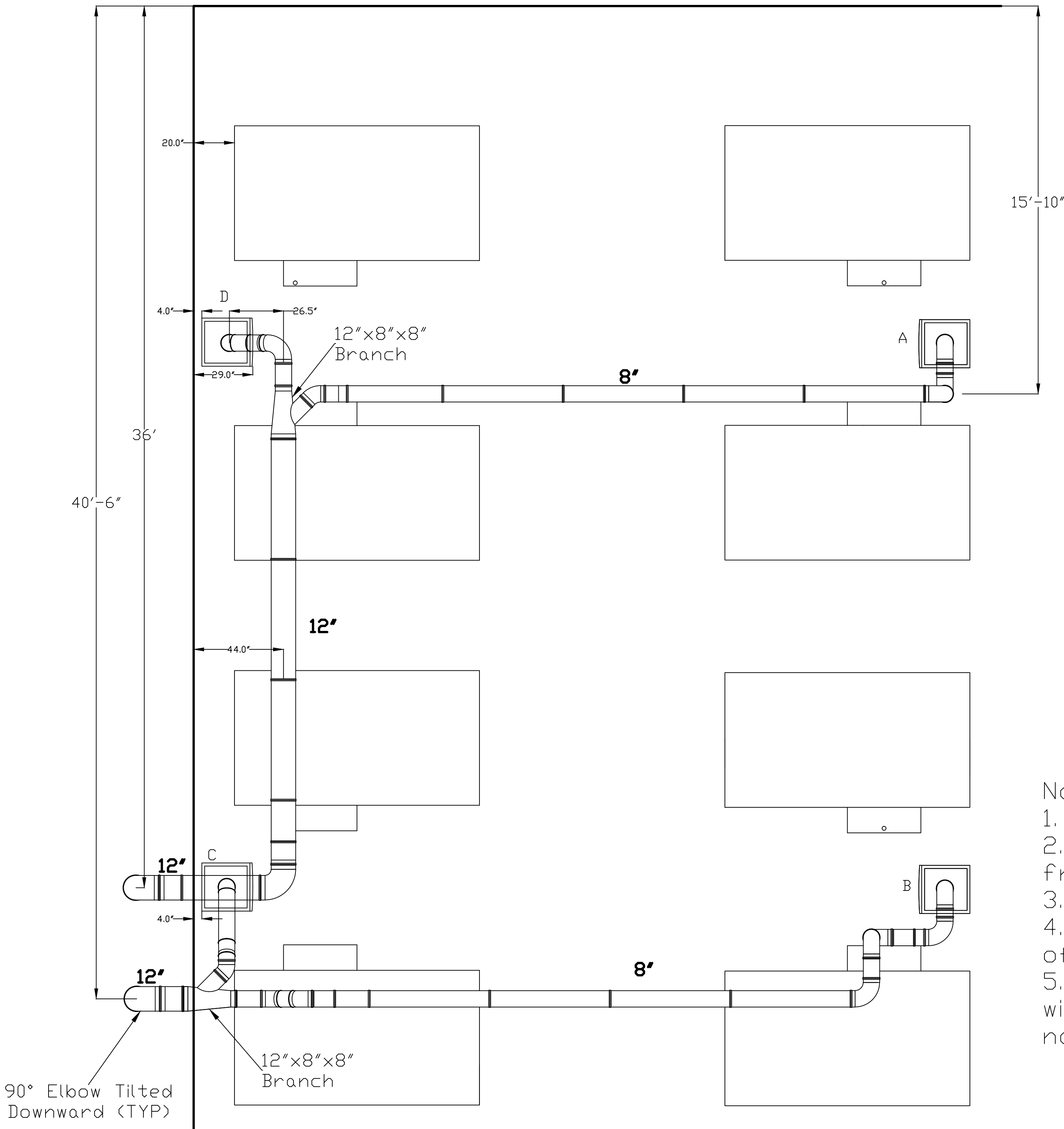
Plan View
