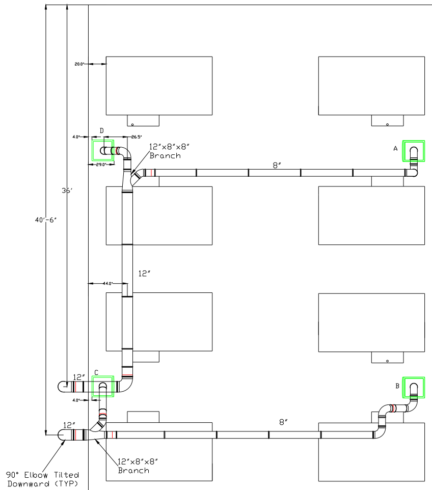
Plan View
