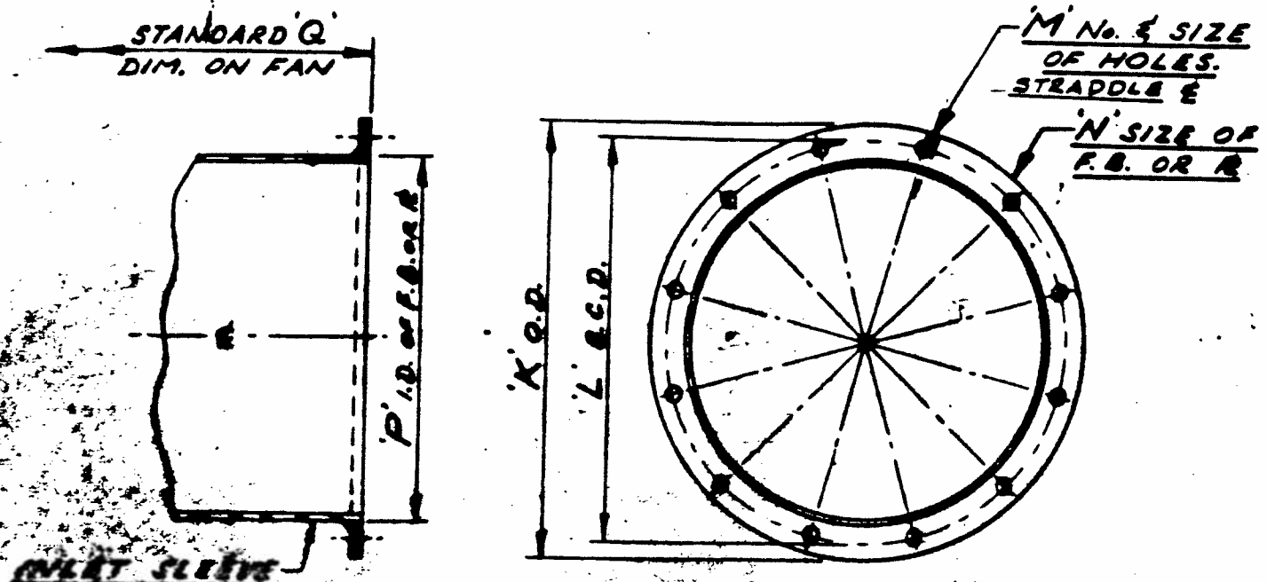
INLET FLANGE
