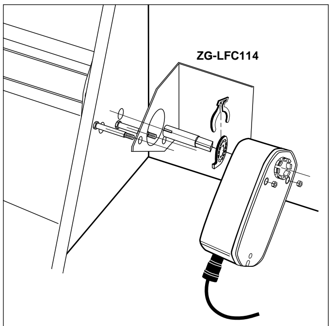
Retrofit solution installation
