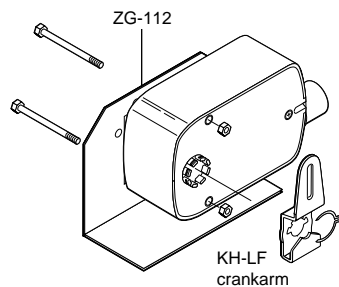
ZG-LF112 Crankarm adaptor kit
