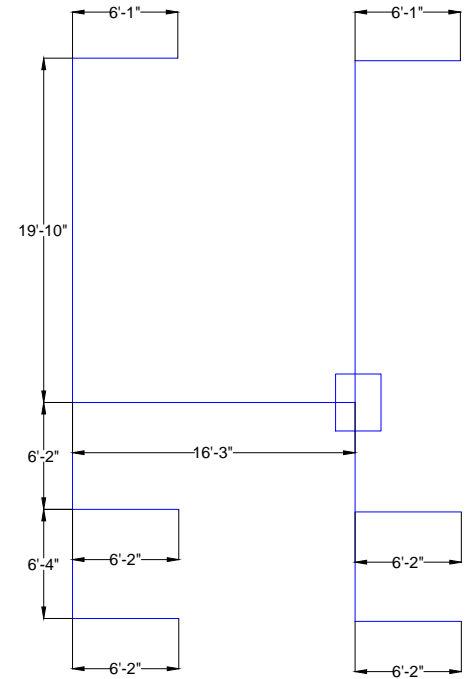
Water Mist Collector
