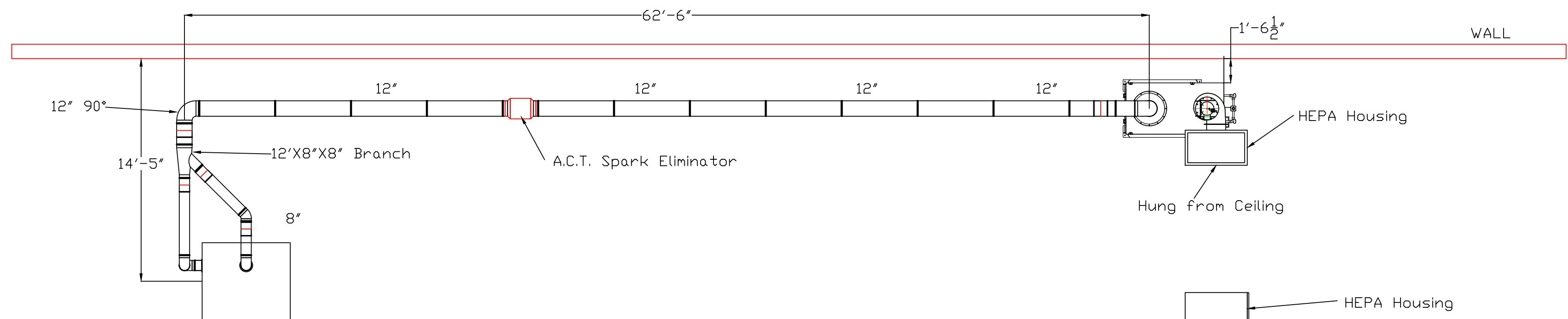
Plan View
