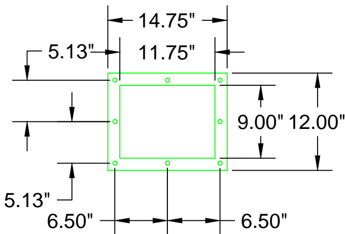
Flange View
