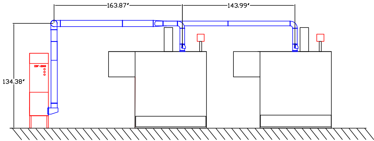
ELEVATION (REAR OF VMP'S 580'S)
