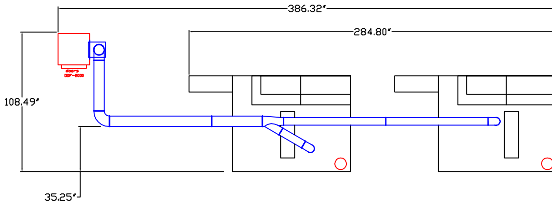
PLAN VIEW
