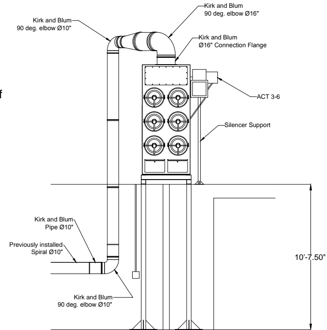
Elevation View
