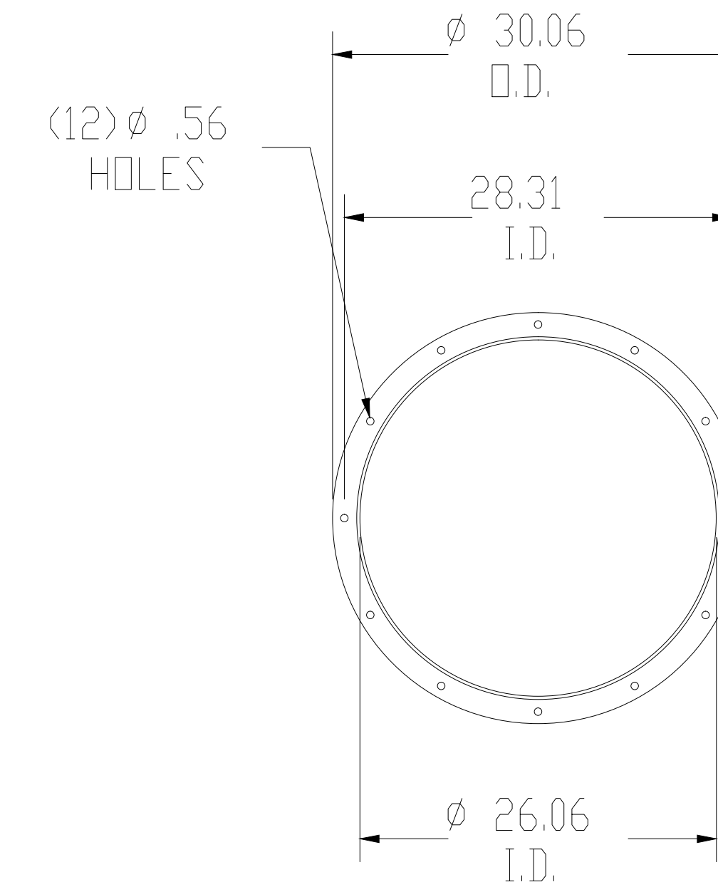
INLET FLANGE DETAIL
