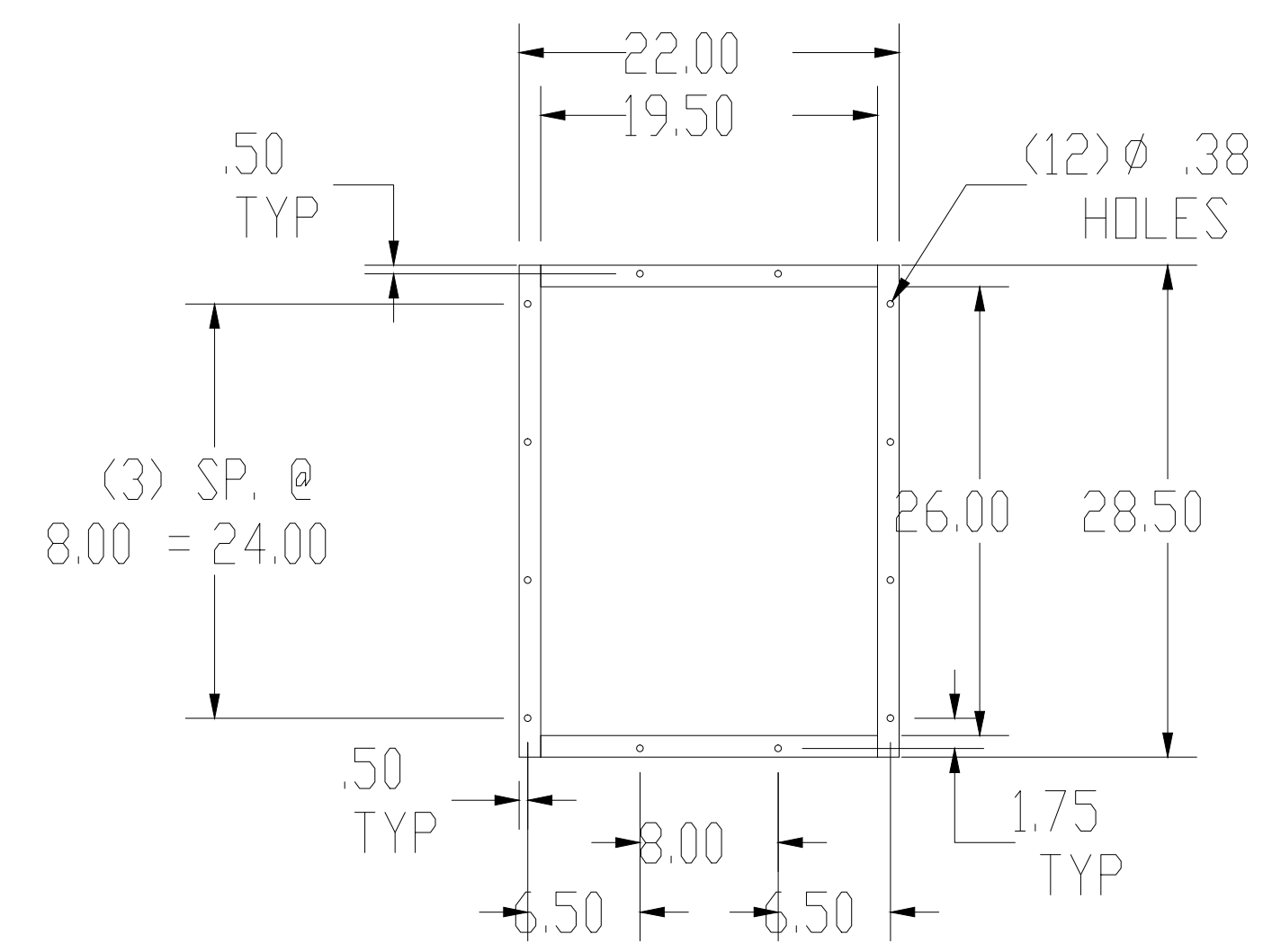
OUTLET FLANGE DETAIL
